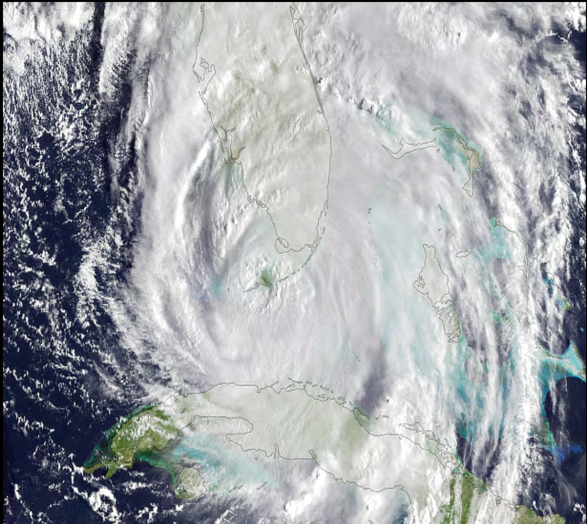
Hurricane Irma Source: NASA
